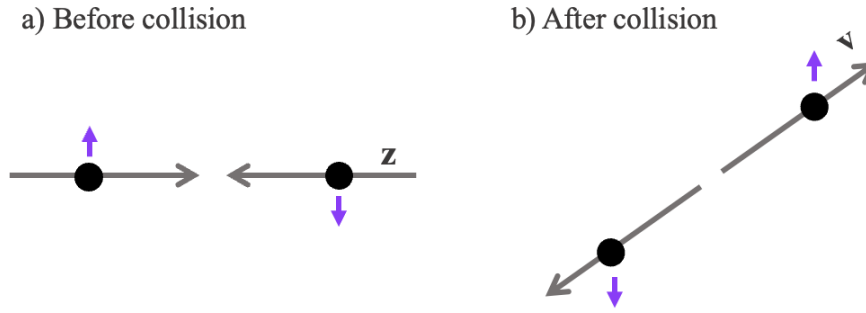
Figure 5.1: Diagram of a collision experiment with no spin interaction ((Cohen-Tannoudji, Diu, Laloe, 1977).)
